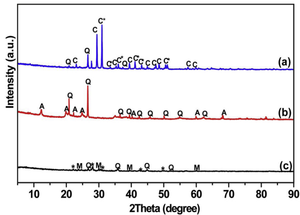
Fig. 4. XRD patterns for coal fly ash (a), clay (b), and the ceramic shell (c) (A: Aluminum silicate hydrate, Q: Quartz, C: Calcium carbonate, C*: Calcium magnesium carbonate, *: Anorthite, M: Calcium magnesium aluminum silicate, and M': Mullite).
