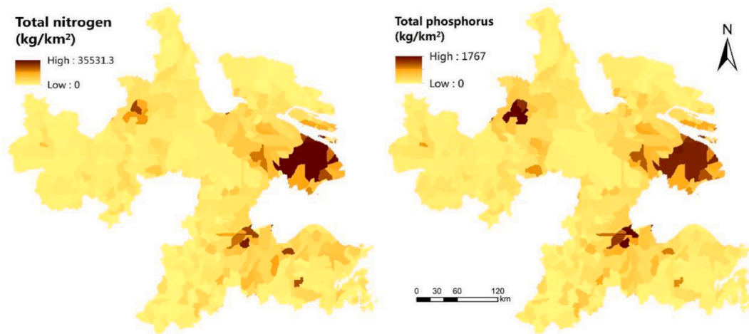
Fig. 5. Total nitrogen and total phosphorus exports of 15 key cities in the Yangtze River Delta region.
